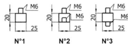
Anti-vibration legs (No. 2 is standard)
