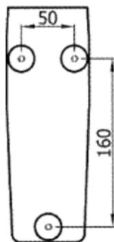
Feet of the types LEV 1, LEX 1 and LES 1
